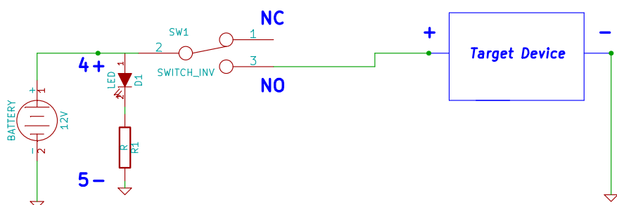
Fig 3 LED is always ON. Device turns ON when switch is pushed.
