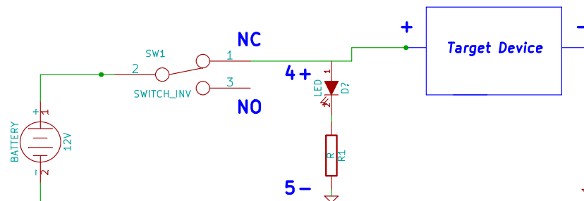
Fig 4 LED turns ON with device. Device turns OFF when switch is pushed.
