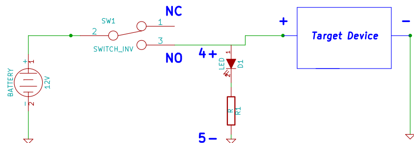
Fig 1 LED turns ON with device. Device turns ON when switch is pushed.
